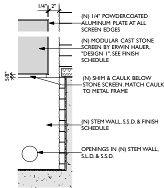
01 SECTION / ELEVATION DETAIL: STONE SCREEN 1 1/2" = 1'-0"
