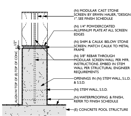
02 SECTION DETAIL: STONE SCREEN 1 1/2" = 1'-0"
